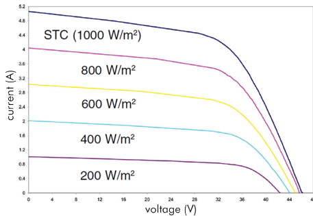
IV Curves at various levels of irradiance at Air Mass 1.5 and 25^{\circ}\text{C} Cell Temperature
